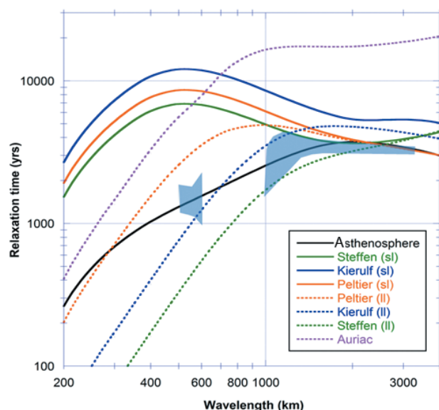
Fig. 1. Relaxation-spectra for the various viscosity models given in Table 1. Curves with solid lines show the relaxation spectra calculated with a thin elastic lithosphere (~30 km), while the dotted lines are for 90–160 km thick elastic lithosphere (according to Table 1). The shaded areas are relaxation spectra (with uncertainties) calculated by McConnell (1968) [16], and inferred by Mitrovica & Peltier [17])
