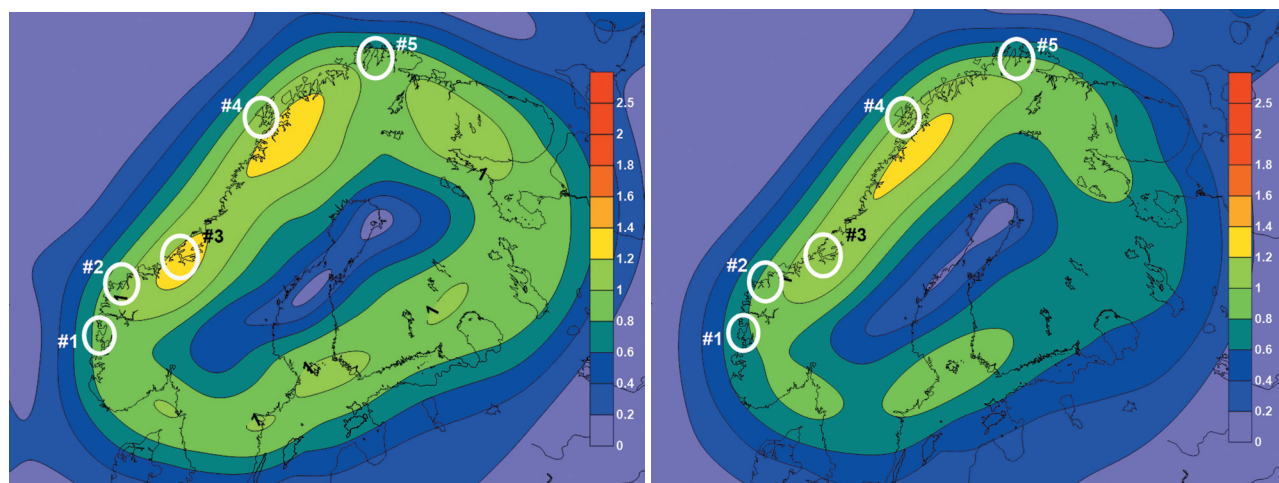
Fig. 10. Calculated shoreline gradients at 12 000 BP; modeled with ICE-5G (Model 4, left) and ICE-6G (Model 5, right), both with upper mantle viscosity 0.5 \times 10^{21} Pa s, lower mantle viscosity 1.7 \times 10^{21} Pa s and lithosphere rigidity 5 \times 10^{24} Nm ( t_e \sim 90 km). Contour interval is 0.2 m/km
